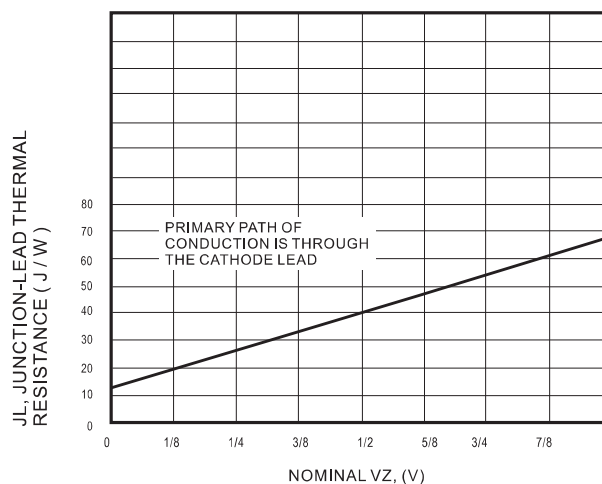
Fig. 9 Typical Thermal Resistance
