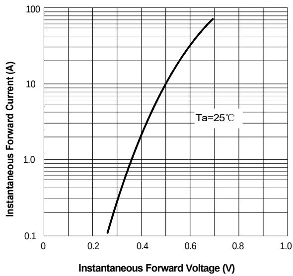
FIG.3: Forward Voltage
