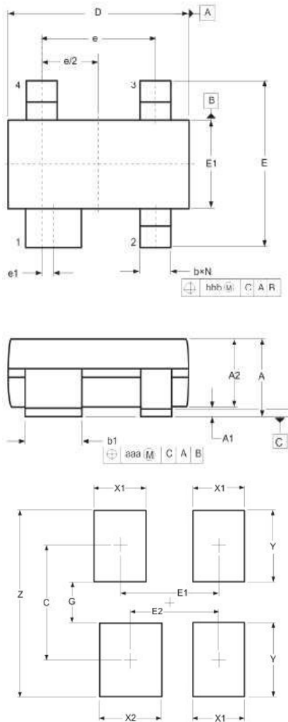
Land Pattern
