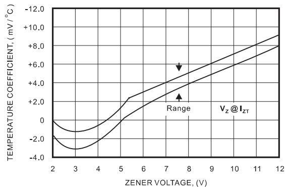
FIG.2A Range for Units to 12 Volts
