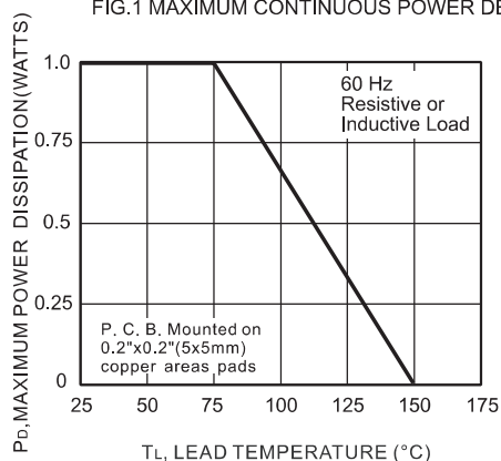
FIG.1 MAXIMUM CONTINUOUS POWER DERATING
