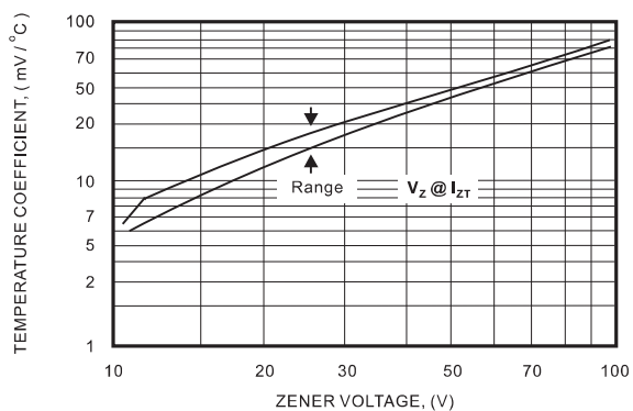
FIG.2B Range for Units to 12 to 100 Volts
