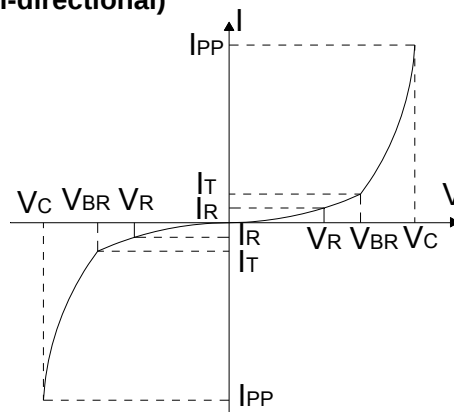
FIG.2: V- I curve characteristics (Bi-directional)
