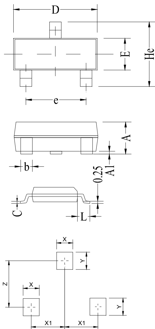
Land Pattern
