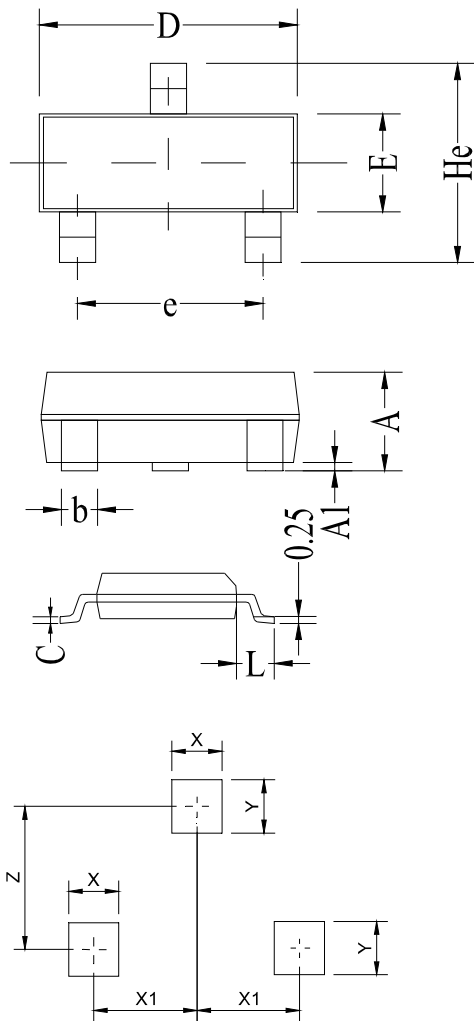
Land Pattern
