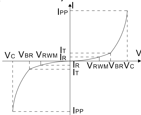
FIG.1: V- I curve characteristics (Bi-directional)
