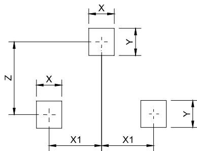
Land Pattern
