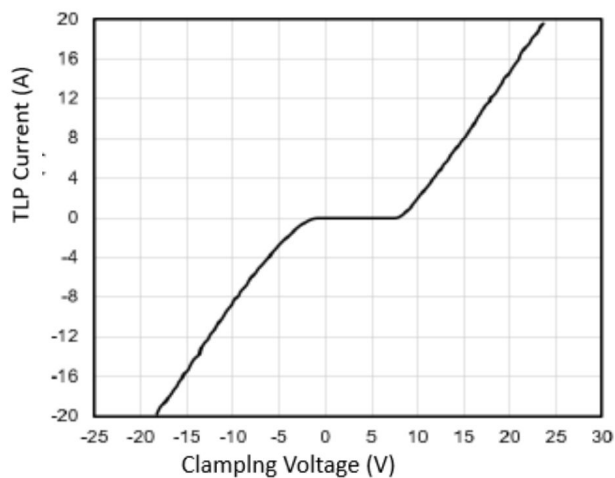
Fig.8 TLP Measurement
