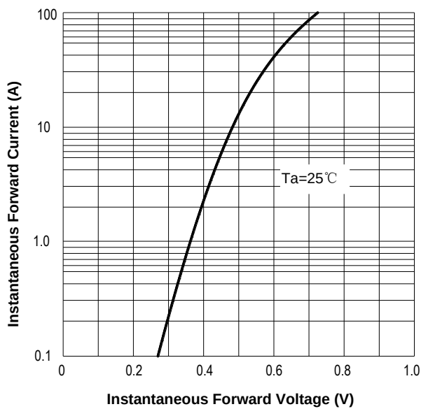
FIG.3: Forward Voltage
