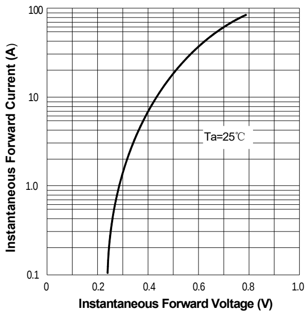
FIG.3: Forward Voltage
