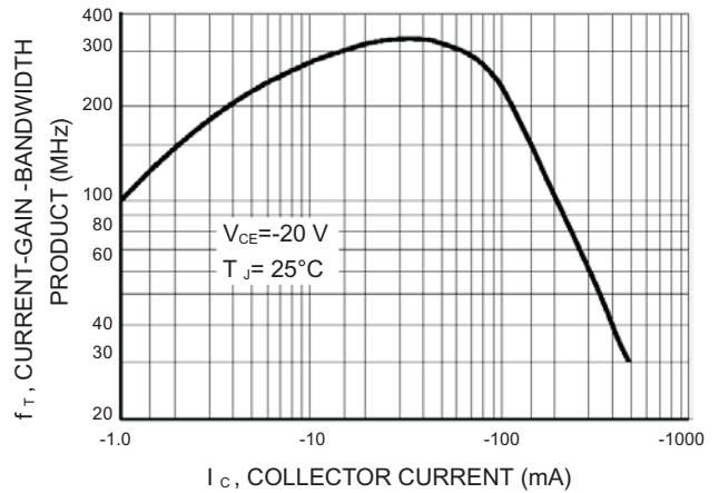
Figure 10. Current-Gain-Bandwidth Product
