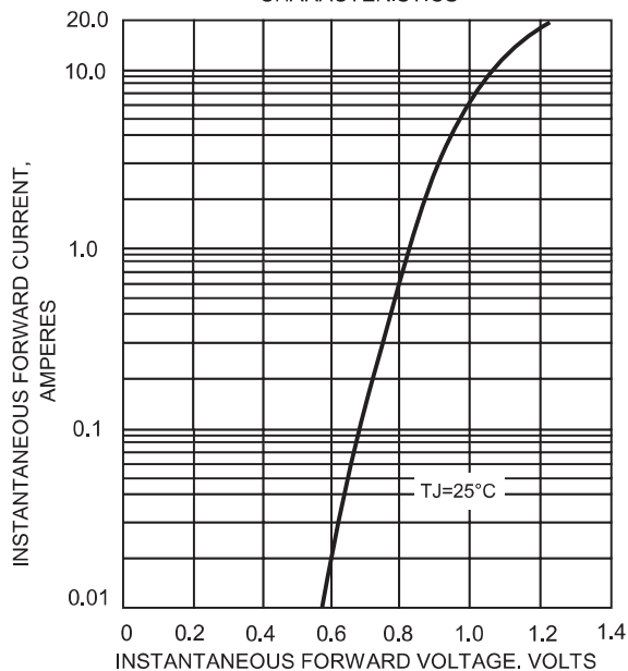
FIG.2-TYPICAL FORWARD CHARACTERISTICS
