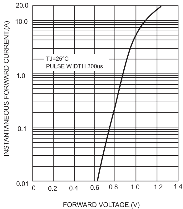
FIG.3-TYPICAL FORWARD CHARACTERISTICS
