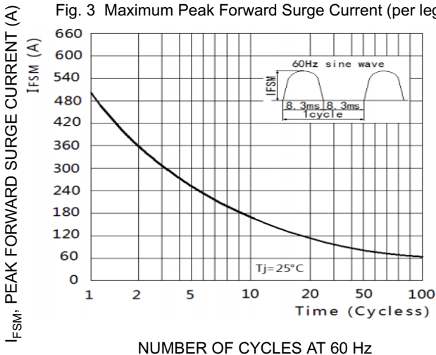
Fig. 3 Maximum Peak Forward Surge Current (per leg)
