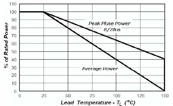
Fig2. Power Derating
