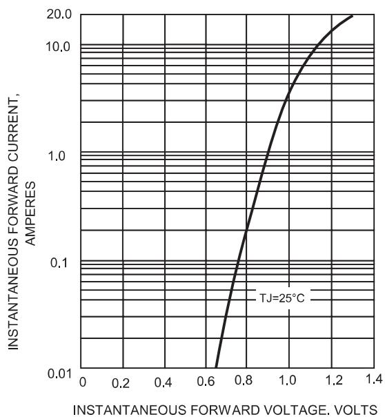
FIG.2-TYPICAL FORWARD CHARACTERISTICS
