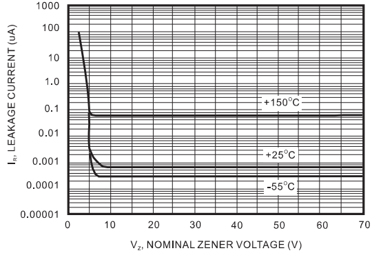
FIG. 4-TYPICAL LEAKAGE CURRENT
