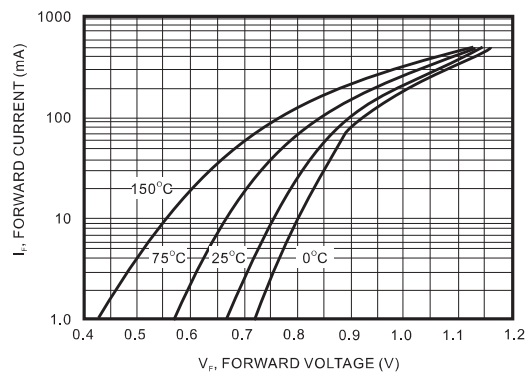
FIG. 2-TYPICAL FORWARD VOLTAGE
