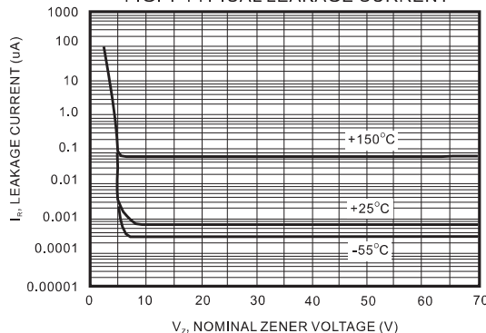
FIG. 4-TYPICAL LEAKAGE CURRENT
