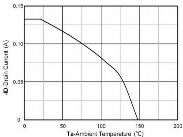
Current dissipation
