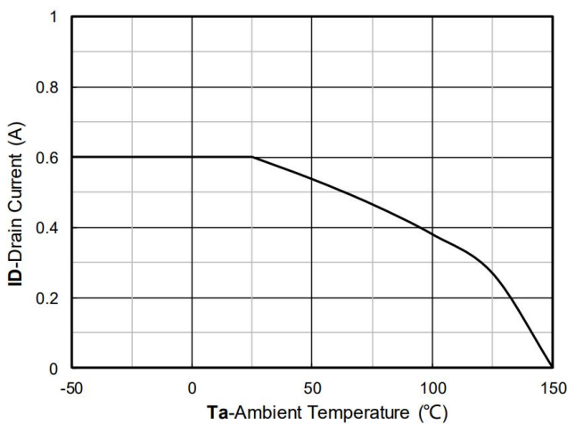
Figure 11. Current dissipation
