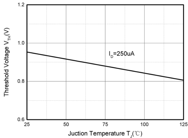
Threshold Voltage
