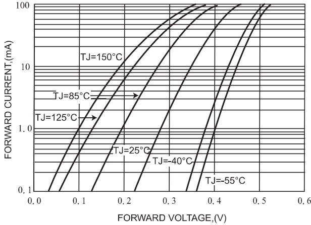
FIG.1-TYPICAL FORWARD CHARACTERISTICS
