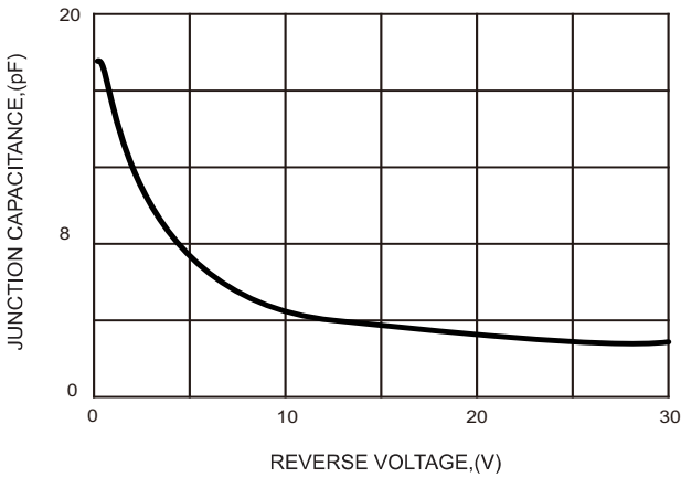
FIG.3-TYPICAL JUNCTION CAPACITANCE
