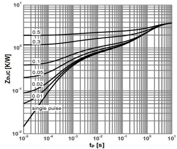
Max. transient thermal impedance
