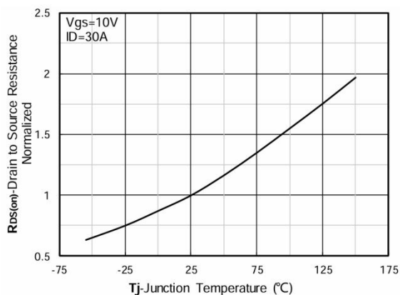
Figure 6. Normalized On-Resistance
