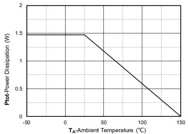
Figure 12. Power dissipation
