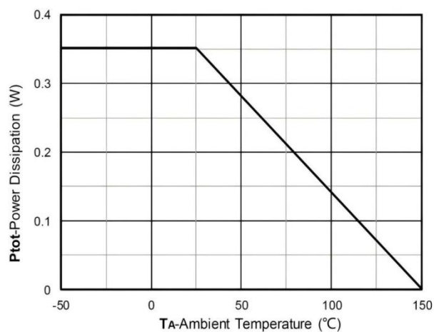
Power dissipation
