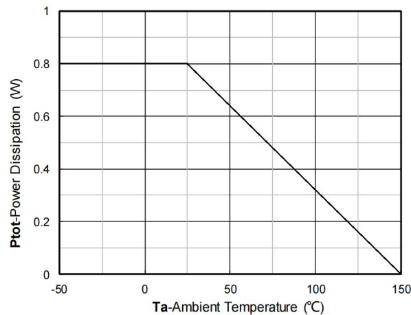
Figure 12. Power dissipation
