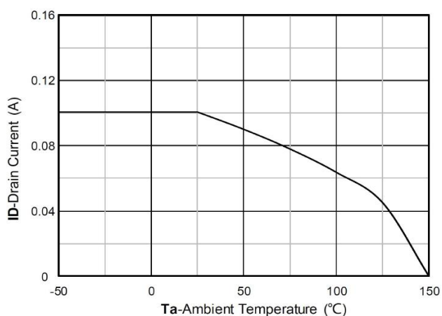
Current dissipation
