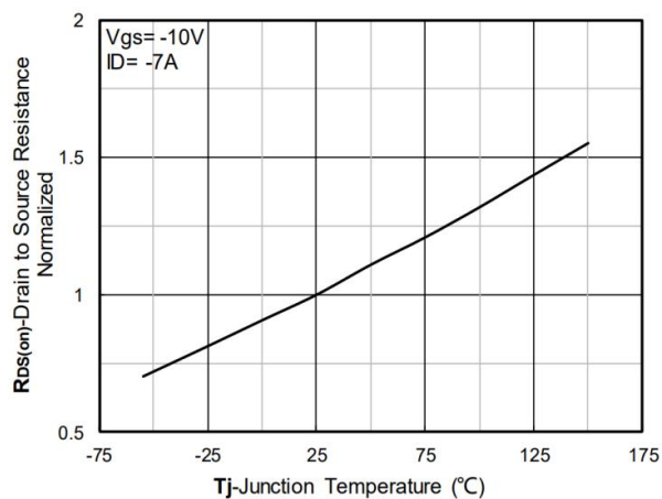
Figure 6. Normalized On-Resistance
