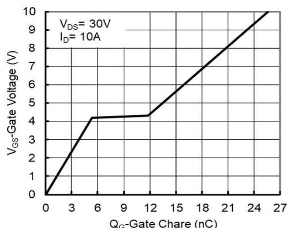
Figure 6. Gate Charge
