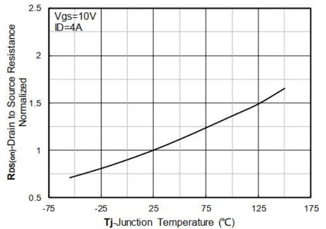
Figure 6. Normalized On-Resistance
