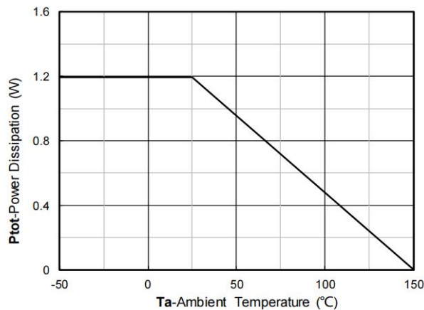
Figure 12. Power dissipation
