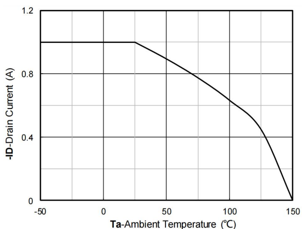
Figure 11. Current dissipation
