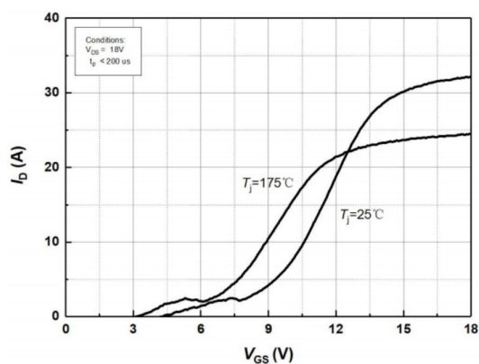
Figure 6. Transfer Characteristics for Various Junction Temperatures
