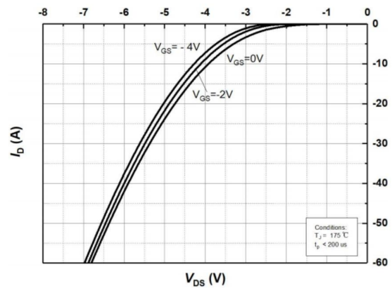
Figure 8. Body Diode Characteristics at T_j=175^{\circ}\text{C}
