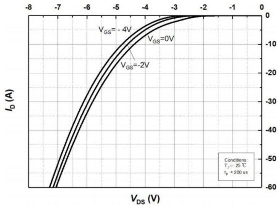
Figure 7. Body Diode Characteristics at T_j=25^{\circ}\text{C}
