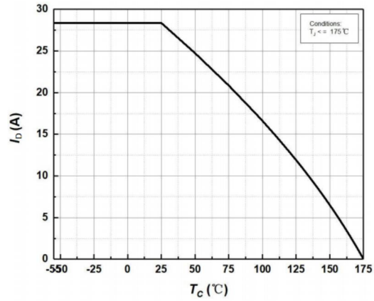
Figure 14. Continuous Drain Current Derating vs Case Temperature
