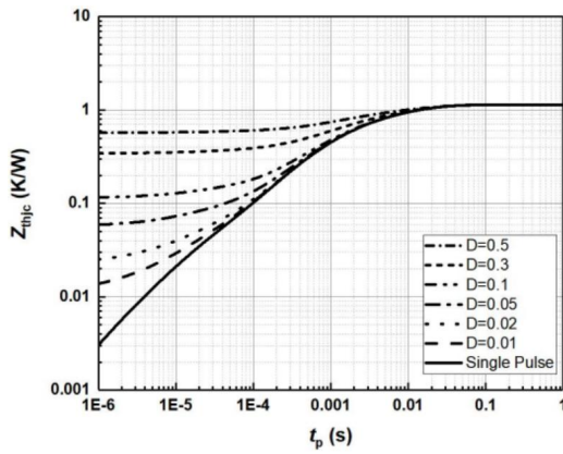
Figure 15. Transient Thermal Impedance (Junction – Case)
