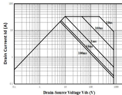
Figure 18. Safe Operating Area
