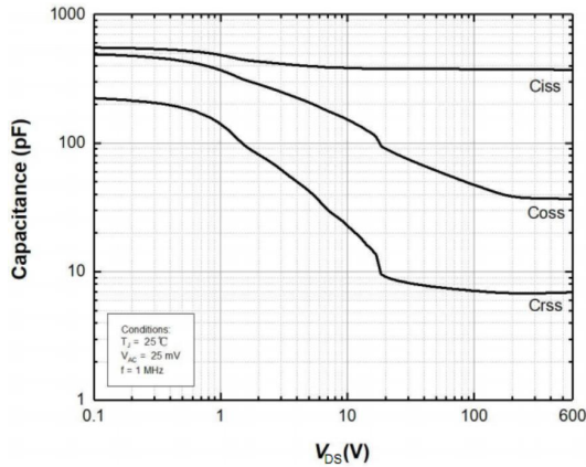
Figure 13. Capacitances vs. Drain-Source Voltage (0 – 1000V)
