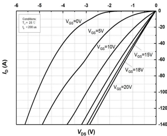
Figure 11. 3rd Quadrant Characteristic at Tj=25°C
