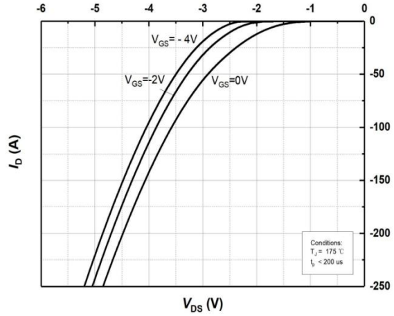
Figure 8. Body Diode Characteristics at T_j=175^\circ\text{C}
