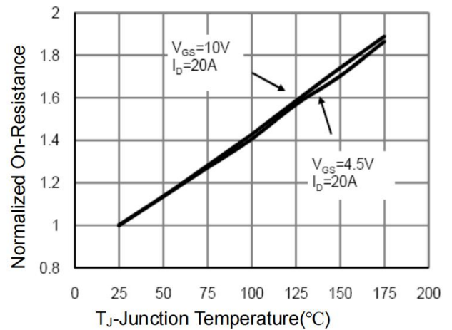
Figure 2 Rdson-Junction Temperature
