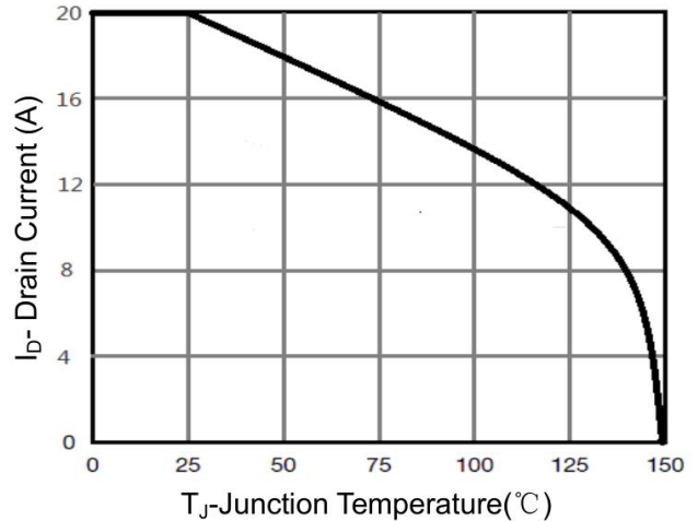
Figure 10 Current De-rating
