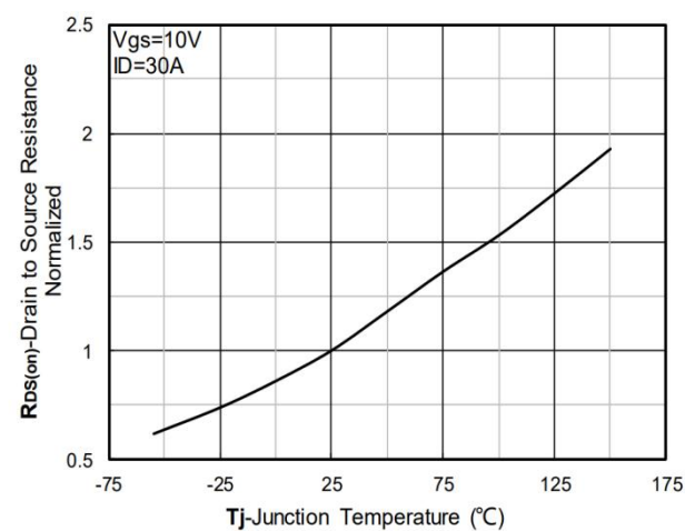
Figure 6. Normalized On-Resistance
