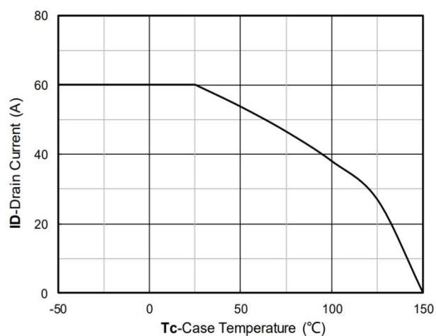
Figure 11. Current dissipation
