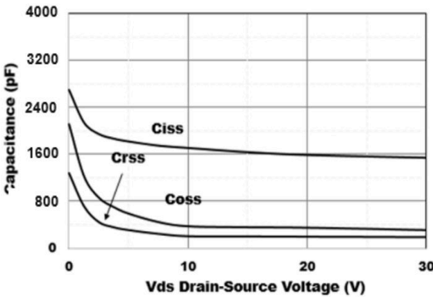
Figure3. Capacitance Characteristics
