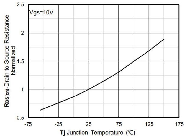
Figure 6. Normalized On-Resistance
