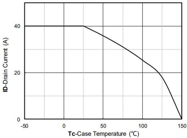
Figure 11. Current dissipation
