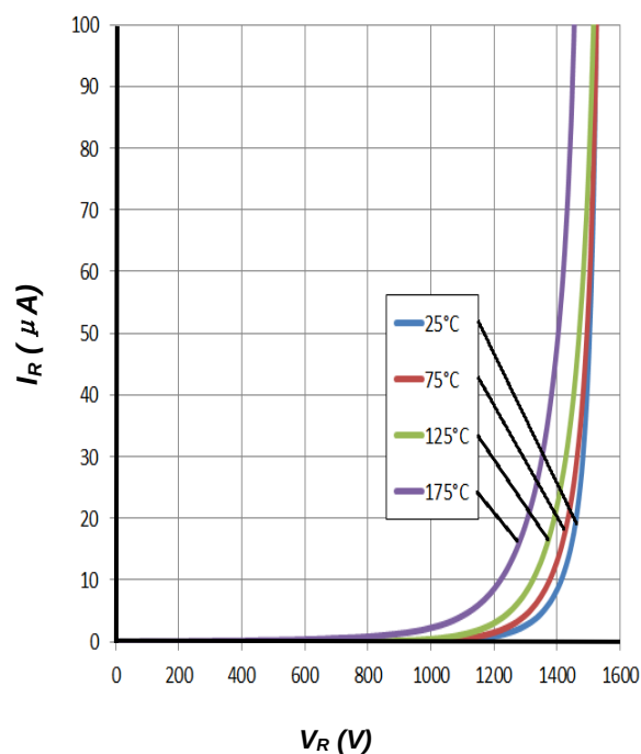
Figure 2. Reverse Characteristics
