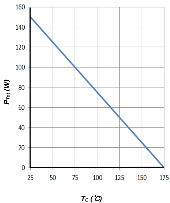
Figure 3. Power Derating
