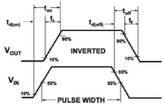
Figure8. Switching wave
