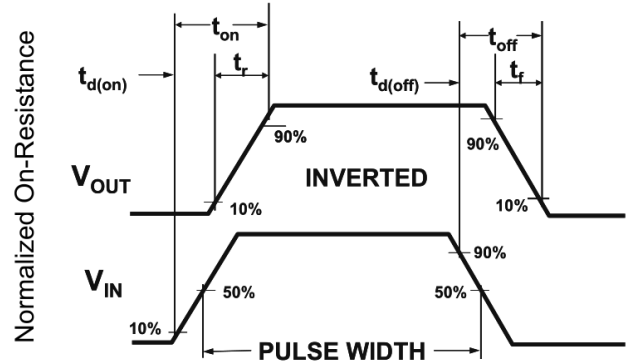
Figure 2: Switching Waveforms
