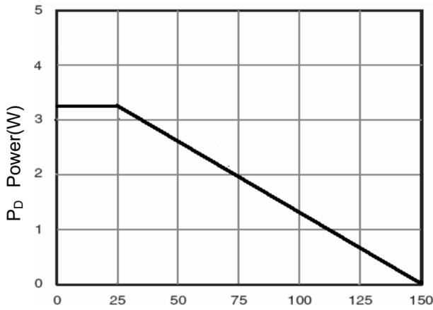
Figure 3 Power Dissipation
