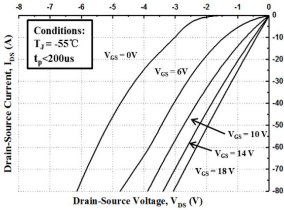
Figure 13. 3rd Quadrant Characteristic at -55°C
