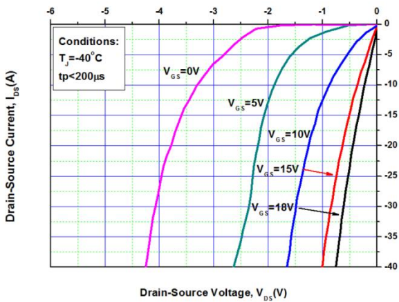
Figure 9. 3rd Quadrant Characteristic at -40°C
