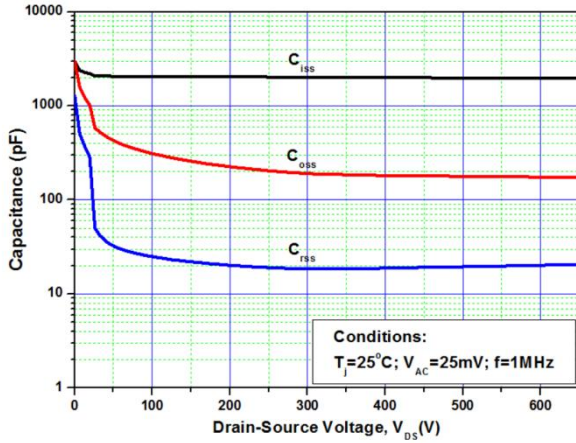
Figure 13. Capacitances vs. Drain-Source Voltage (0 - 650V)
