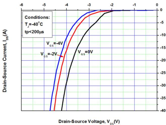
Figure 5. Body Diode Characteristic at -40^\circ\text{C}
