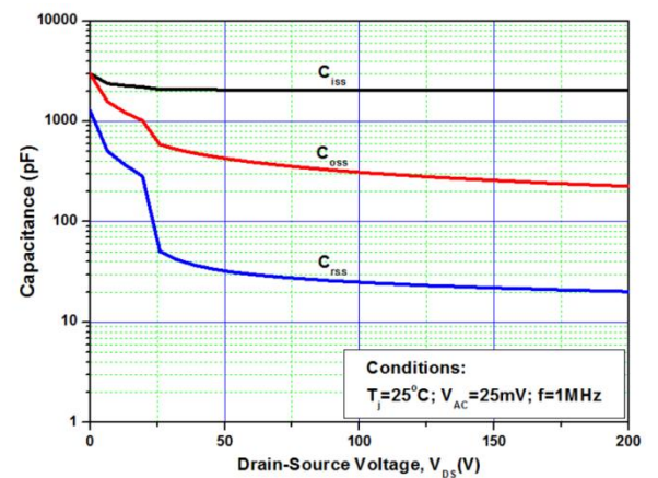
Figure 12. Capacitances vs. Drain-Source Voltage (0 - 200V)
