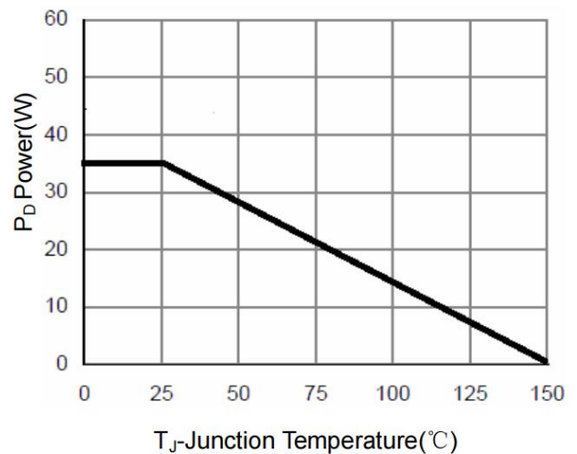
Figure 6 Power Dissipation
