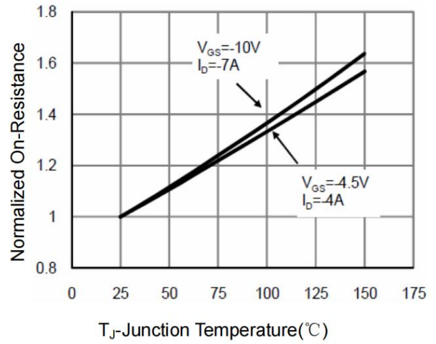
Figure 2 Rdson-Junction Temperature
