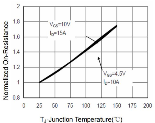
Figure 4 Drain-Source On-Resistance
