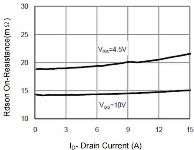
Figure 3 Drain-Source On-Resistance
