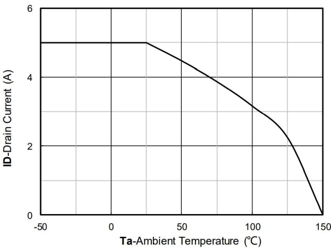
Figure 11. Current dissipation
