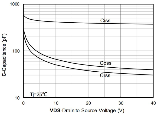
Figure 3. Capacitance Characteristics
