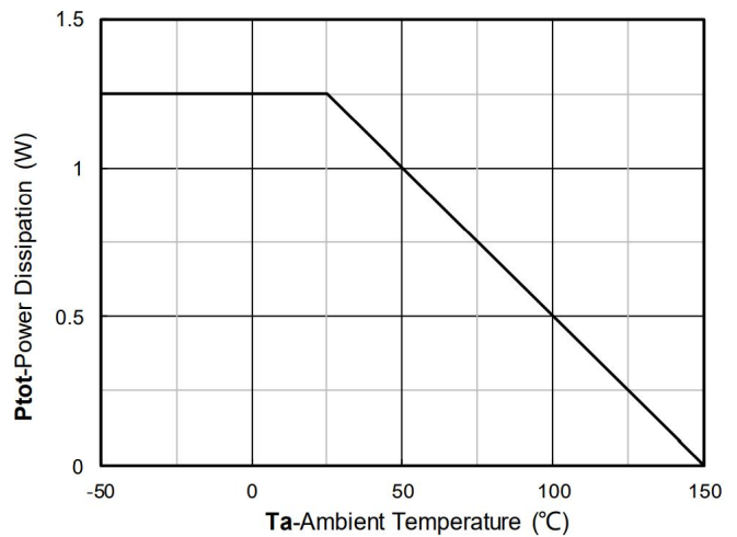
Figure 12. Power dissipation
