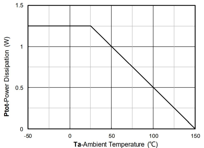
Figure 12. Power dissipation
